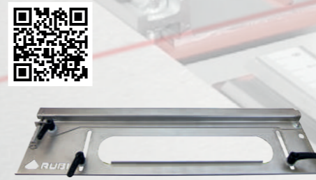
SKIRTING LATERAL STOP Ref. 51910 FOR: DC-250, DS-250, DX-250 PLUS, DX-350
